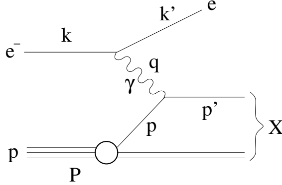
Figure 3: Deep inelastic scattering.
