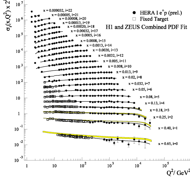
Figure 4: Predictions for deep inelastic scattering compared to data.
