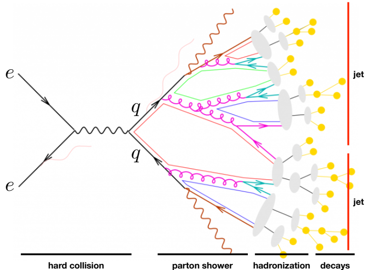
Figure 2: Schematic depiction of a hard e^+e^- \rightarrow q\bar{q} event with subsequent parton shower, hadronization, and hadron decays. The collimated sprays of particles that emerge are called jets. Image from Ref. [8].
