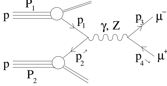
Figure 5: Drell-Yan production of \mu^+\mu^- in a pp collision.
